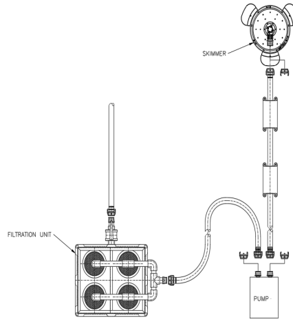
Above: Skimmer system layout
